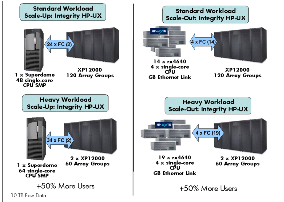
Figure 3: HP 10TB HP-UX reference configurations for Oracle
